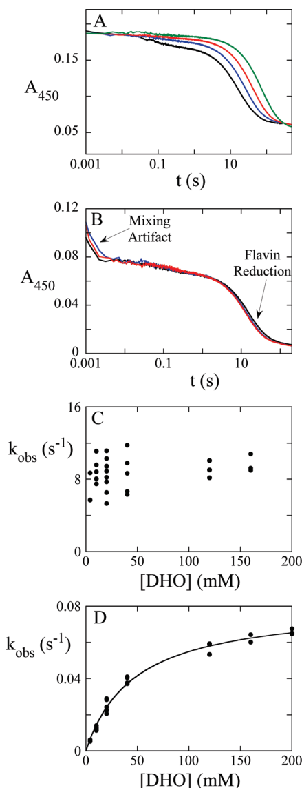
FIGURE 6: Reductive half-reaction of the Asn246Ala mutant DHOD. (A) Reaction traces observed when \sim 29 \mu\text{M} enzyme (before mixing) was mixed with 20–48 mM DHO (before mixing), pH 8.5 at 4 °C. The instrument dead time (1 ms) has not been added to the times recorded in the traces. (B) Reaction traces observed when \sim 12 \mu\text{M} enzyme (before mixing) was mixed with 240–400 mM DHO (before mixing), pH 8.5 at 4 °C. The mixing artifact is followed by two phases. The large second phase represents flavin reduction. (C) The observed rate constant of the first phase after the mixing artifact is independent of DHO concentration, with a k_{\text{obs}} scattered around \sim 9 \text{ s}^{-1} . (D) The observed rate constant of the flavin reduction phase saturates with increasing DHO concentration, giving a k_{\text{red}} of 0.081 \pm 0.002 \text{ s}^{-1} and an apparent K_d of DHO of 47 \pm 3 \text{ mM} .
