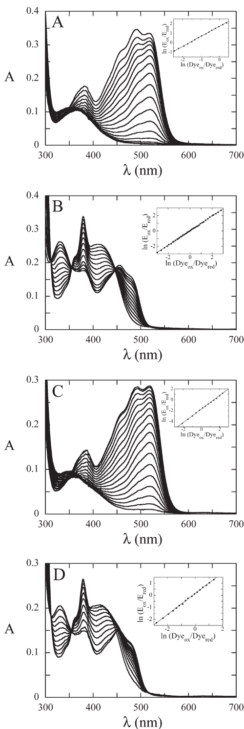
FIGURE 2: Determination of reduction potentials. Reduction potentials were determined using the xanthine/xanthine oxidase method of Massey (17) in 0.1 M NaPi, pH 7 at 25 °C. The reduction potential of wild-type E. coli DHOD was determined using phenosafranin (A) and 1-anthraquinone sulfonate (B). The reduction potential of the Asn246Ala mutant enzyme was also determined using phenosafranin (C) and 1-anthraquinone sulfonate (D). The insets in each panel show the Nernst plot for determining the potentials.
