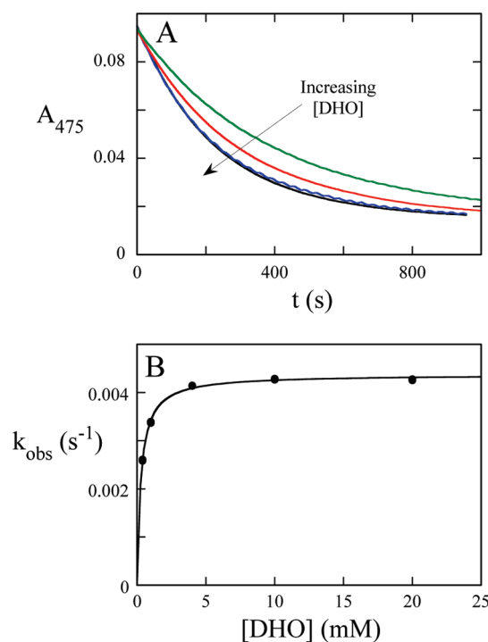
FIGURE 5: Reductive half-reaction of the Asn172Ala mutant DHOD. (A) Reaction traces at 475 nm observed when \sim 14 \mu M enzyme (before mixing) was mixed with DHO ranging from 0.8 to 40 mM (before mixing), pH 8.5 at 4 °C. The instrument dead time (1 ms) has not been added to the times recorded in the traces. (B) The observed rate constant varies hyperbolically with DHO concentration giving a k_{red} of 0.00437 \pm 0.0002 s^{-1} and a K_{d,DHO} of 278 \pm 9 \mu M .
