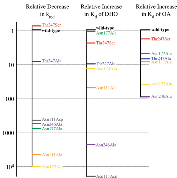
FIGURE 7: Relative effects of all mutations. The effects of each mutation on the K_d of OA, the K_d of DHO, and the reduction rate constant with respect to wild type are shown.
