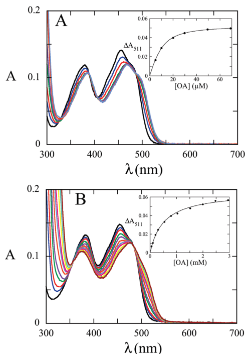
FIGURE 3: OA binding titration, pH 8.5, at 25 °C. The Thr247Ser mutant enzyme (A) and the Asn246Ala mutant enzyme (B) were titrated aerobically with OA. The insets show the maximum change in absorbance due to OA binding as a function of OA concentration. Fitting to eq 1 gives a K_d of 3.8 \pm 0.5 \mu M for Thr247Ser (A). Fitting to a square hyperbola gives a K_d value of 520 \pm 30 \mu M for Asn246Ala (B).
