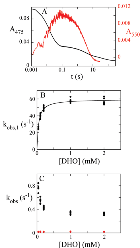
FIGURE 4: Reductive half-reaction of the Thr247Ser mutant DHOD. (A) Reaction traces observed when \sim 15 \mu M enzyme (before mixing) equilibrated in 0.1 M Tris, pH 8.5, was mixed with 4 mM DHO (before mixing) at 4 °C. At 475 nm (black), the reaction occurs in three phases. The first (large) phase represents the chemical step. The second phase represents product release. At 550 nm (red), flavin reduction is seen as an increase in absorbance, and product dissociation is seen as a decrease in absorbance. The instrument dead time (1 ms) has not been added to the times recorded in the traces. (B) The observed rate constant of the first phase (flavin reduction) saturates with increasing DHO concentration, giving a reduction rate constant ( k_{red} ) of 58.8 \pm 1.1 s^{-1} and a K_{d,DHO} of 45 \pm 5 \mu M . (C) Concentration dependence of the observed rate constant for the second and third phases. The observed rate constant of the second phase (black), OA release, decreases with increasing DHO concentration, giving a limiting value of 0.37 s^{-1} . The observed rate constant of the final phase (red) is \sim 0.02 s^{-1} and is independent of DHO concentration.
